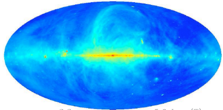
Sky at 100 MHz
