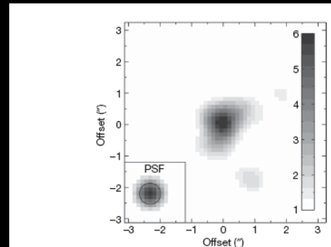
Figure 2 | Ly \alpha line image of UDFy-38135539. The line image
