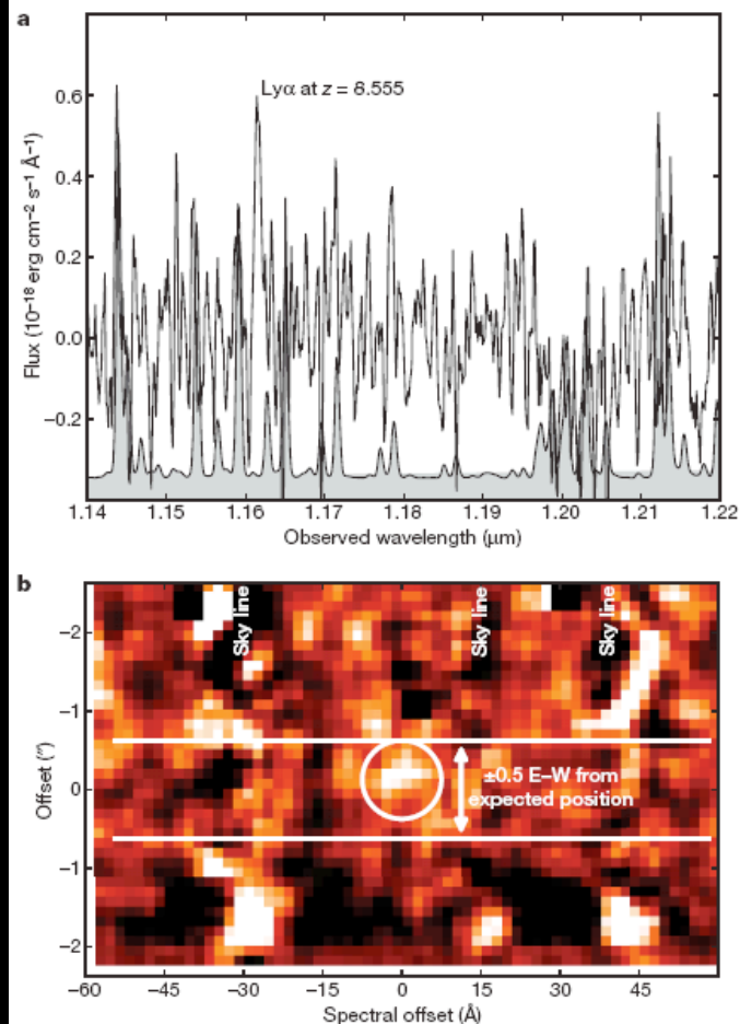
Figure 1 | Two representations of the spectrum of UDFy-38135539 showing its significance. a, The spectrum shows a faint emission line detected at 6\sigma
